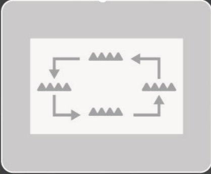
Box Feeding System The feed dogs move in a square which results in better feeding capability
